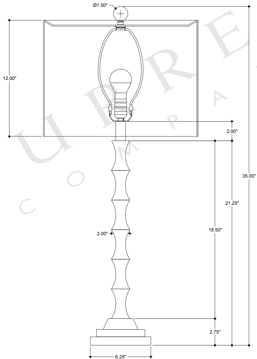
FRONT VIEW
